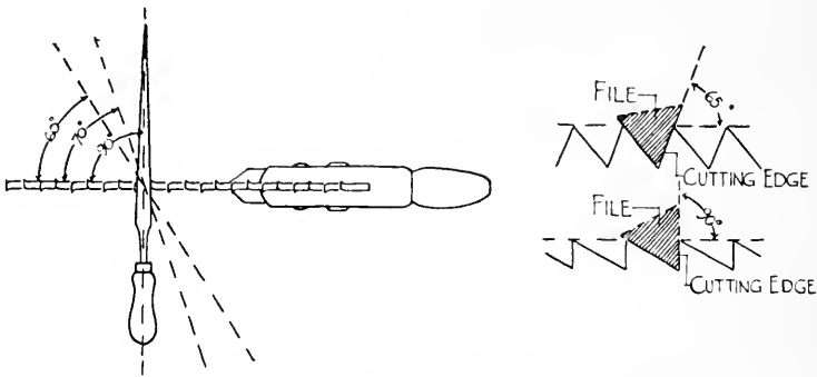
FIG. 114. FILING POSITIONS FOR CROSSCUT AND RIP-SAW TEETH.
